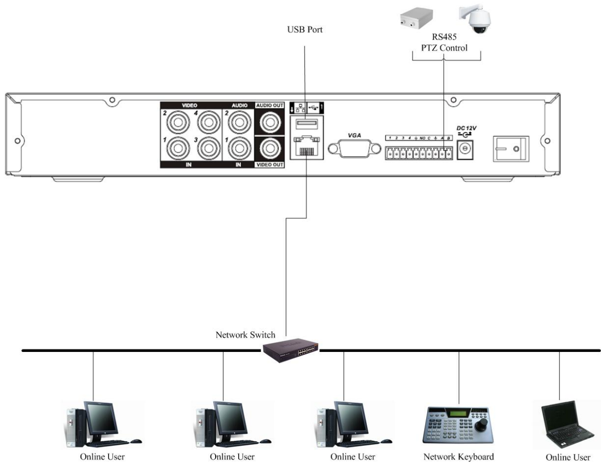
Figure 3-17 Simple Entry Level Series
